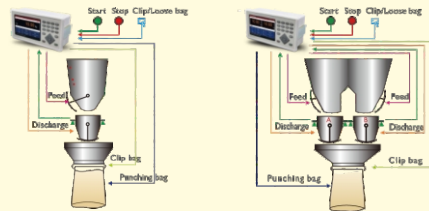
Bagging Process
