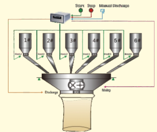
Batching Process
