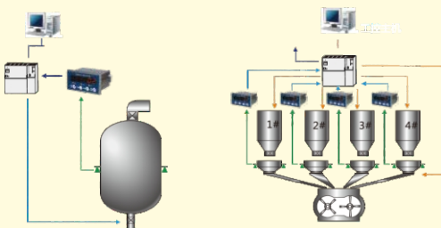
Weighing Process
